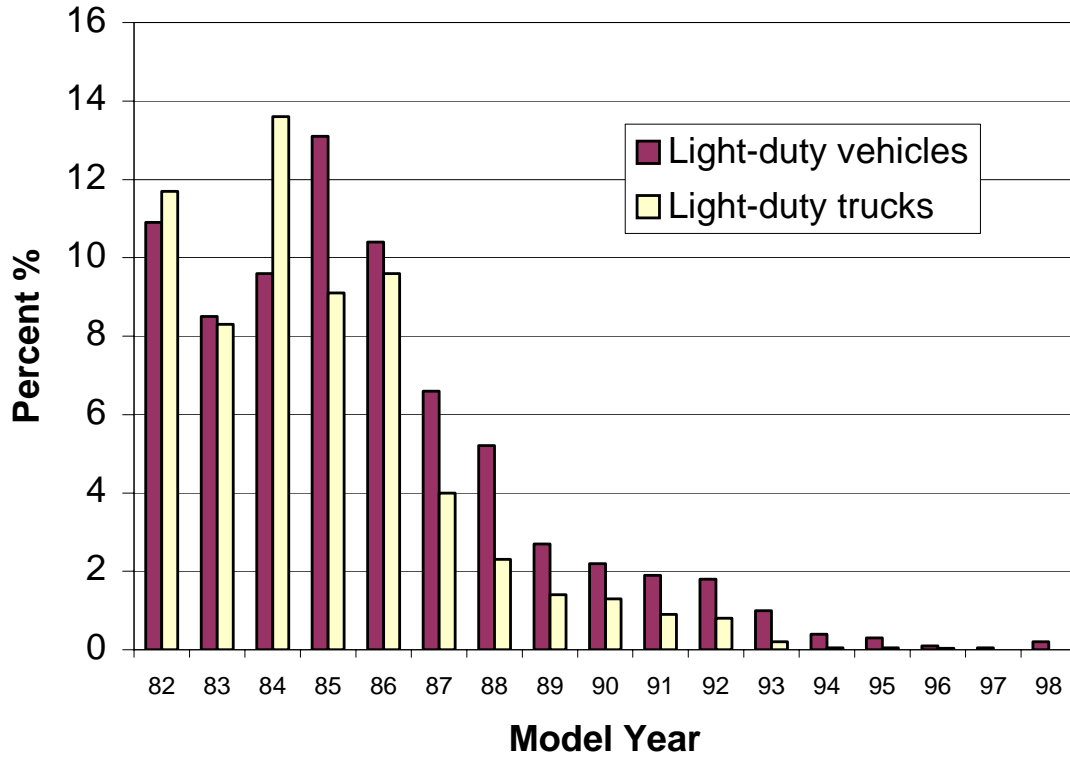
Figure 1. Emissions (CO, HC and NOx) Failure Rate in the Colorado I/M240 program during 1997. Data are from CDPHE 1998 report 3 .
