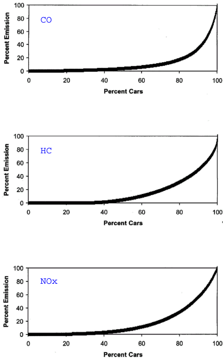
Figure 3. Cumulative curves of three pollutants measured by remote sensing in Denver in 1998/99. Note that 50% of the fleet is essentially eligible.
